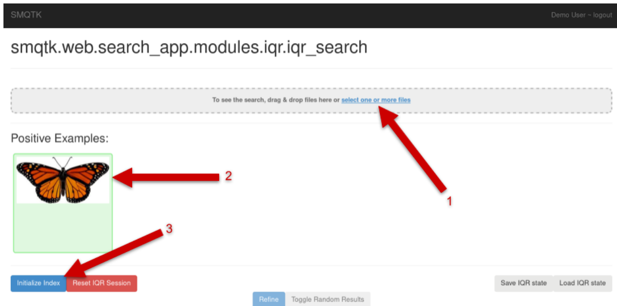
Fig. 5: IQR Initialization
